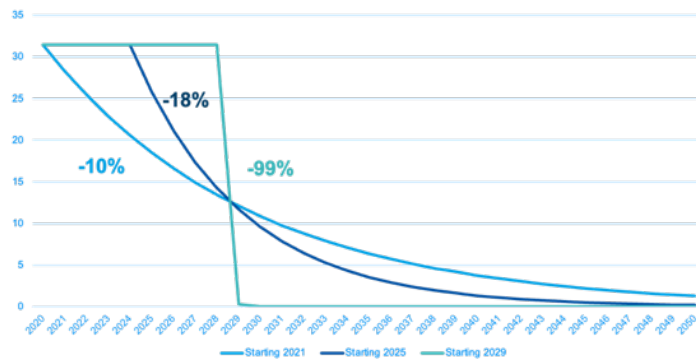
Figure 5: Impact of starting date on carbon pathways
