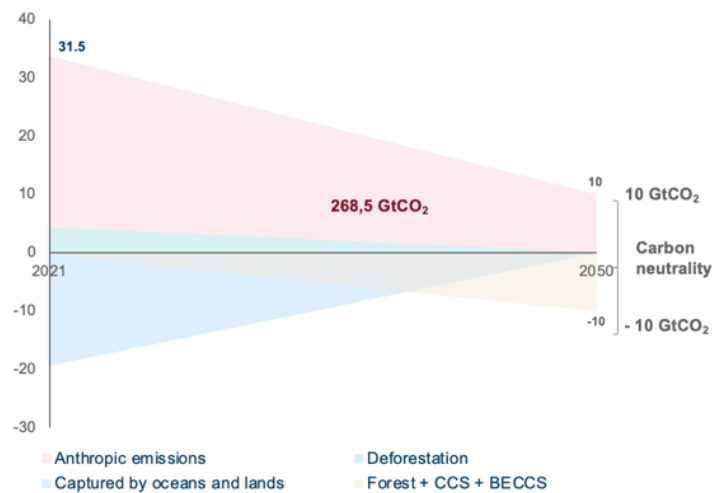
Figure 1: Reduction trajectory to net zero emissions based on carbon budget
